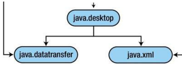
Figure 4-13. The module graph of myModule
