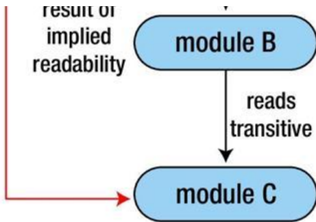
Figure 4-11. Module graph showing implied readability
