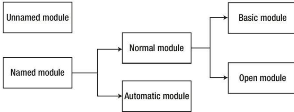
Figure 4-15. The classification of modules in the JPMS
