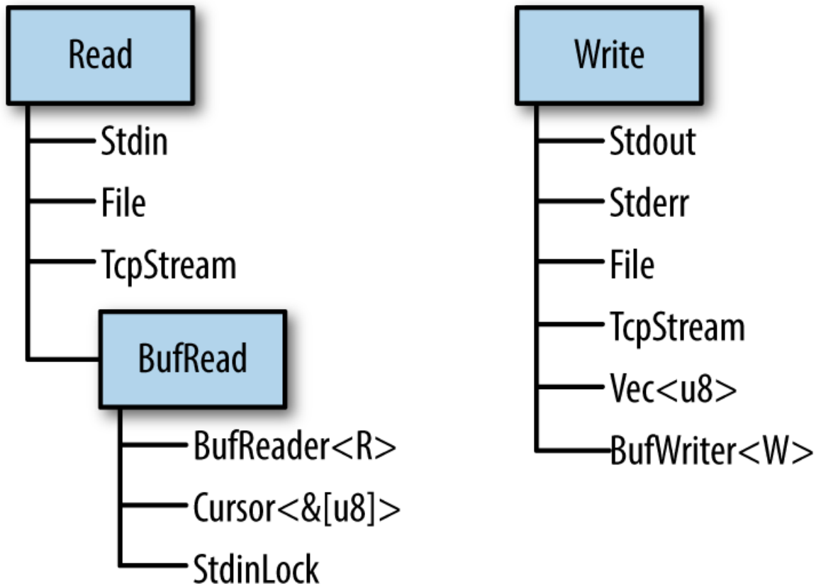
Figure 18-1. Selected reader and writer types from the Rust standard library
