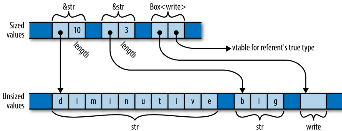
Figure 13-1. References to unsized values
