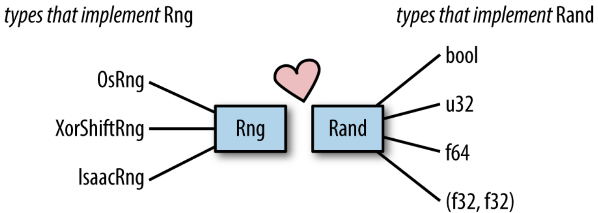
Figure 11-3. Buddy traits illustrated. The Rng types listed on the left are real random number generators provided by the rand crate.
