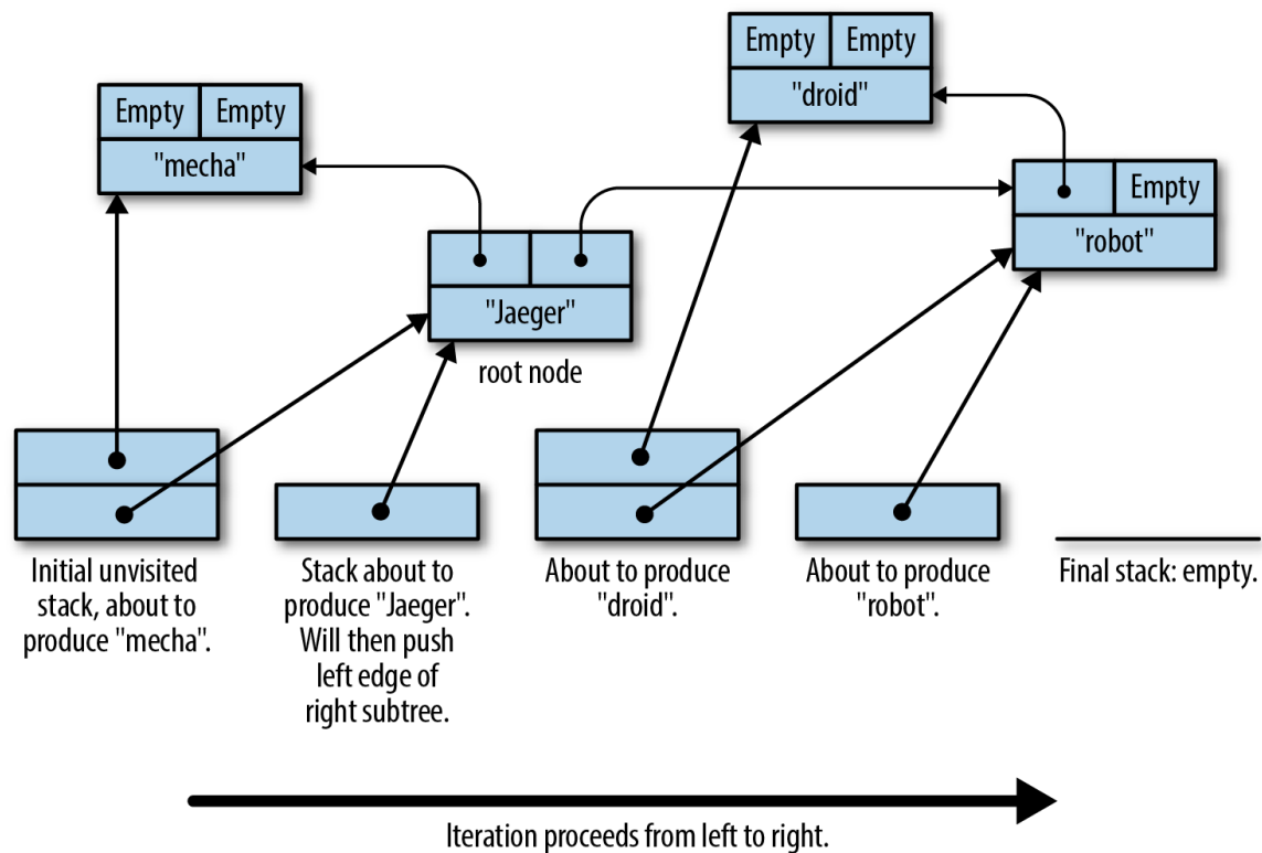
Figure 15-1. Iterating over a binary tree
