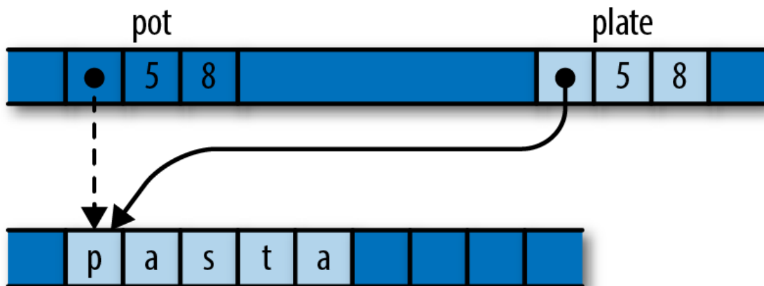
Figure 21-2. Moving a string from one local variable to another
