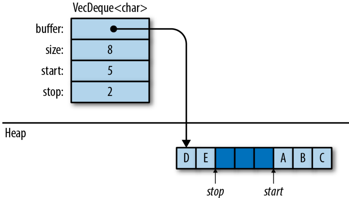
Figure 16-3. How a VecDeque is stored in memory
