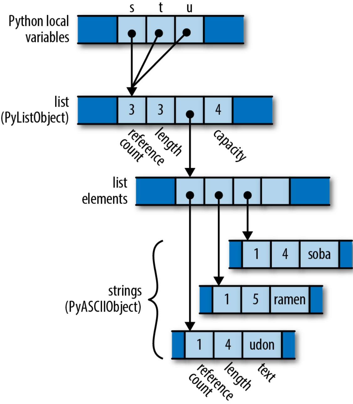
Figure 4-6. The result of assigning s to both t and u in Python
