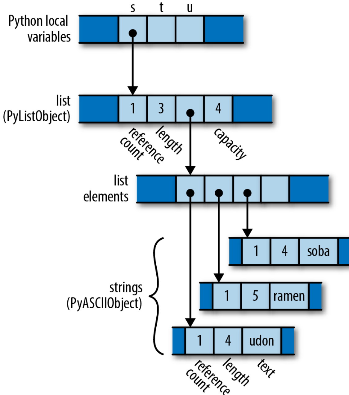
Figure 4-5. How Python represents a list of strings in memory
