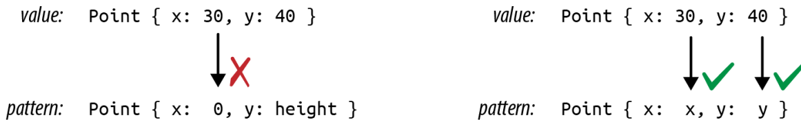
Figure 10-6. Pattern matching with structs
