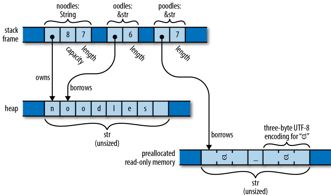
Figure 3-3. String , &str , and str
