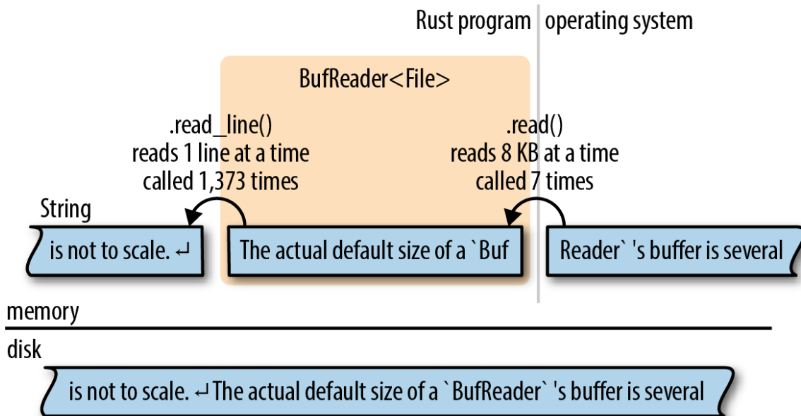
Figure 18-2. A buffered file reader
