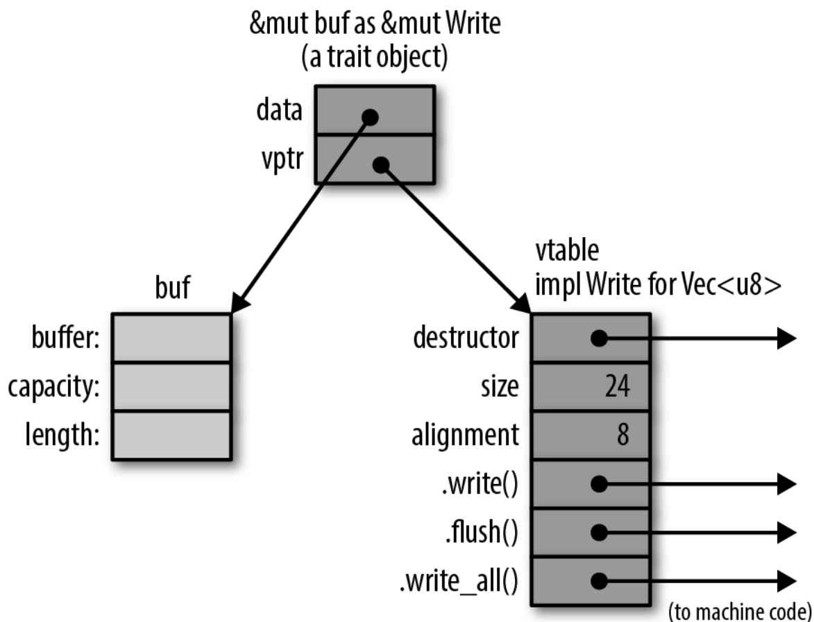
Figure 11-1. Trait objects in memory
