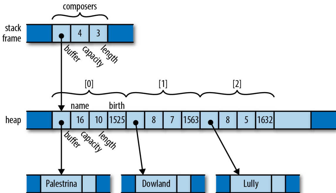
Figure 4-4. A more complex tree of ownership
