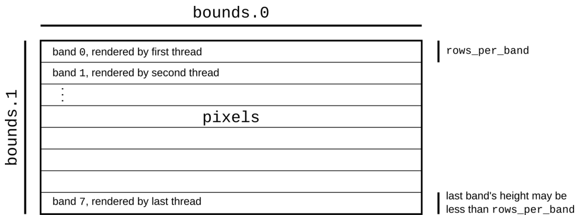
Figure 2-6. Dividing the pixel buffer into bands for parallel rendering
