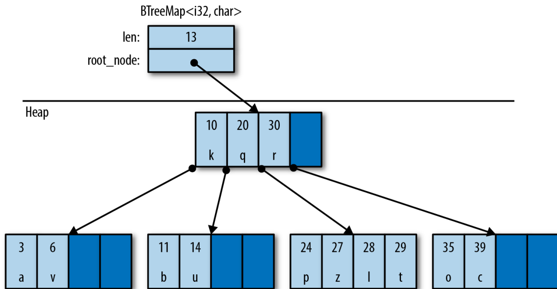
Figure 16-6. A BTreeMap in memory
