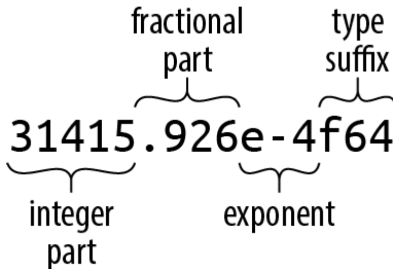
Figure 3-1. A floating-point literal
