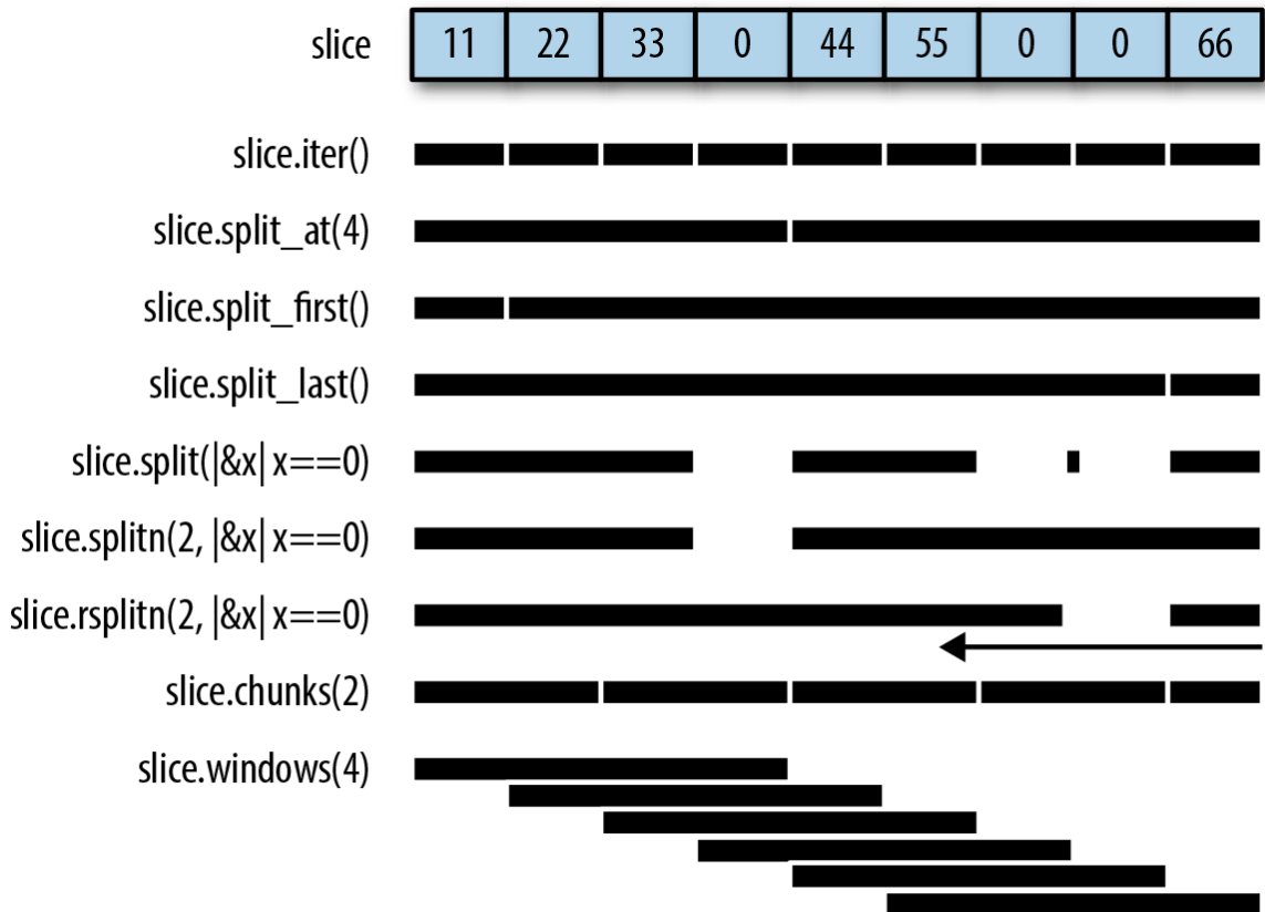
Figure 16-2. Splitting methods illustrated. The little rectangle in the output of slice.split() is an empty slice, caused by the two adjacent separators. Also note that rspln produces its output in end-to-start order, unlike all the others.
