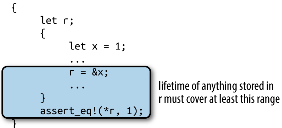
Figure 5-4. Permissible lifetimes for reference stored in r
