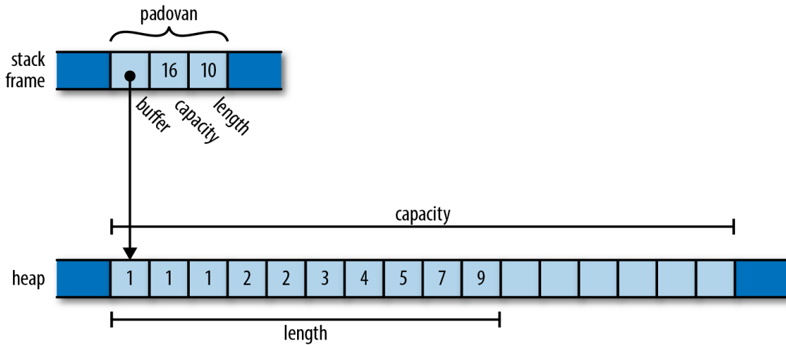
Figure 4-2. A Vec32 on the stack, pointing to its buffer in the heap
