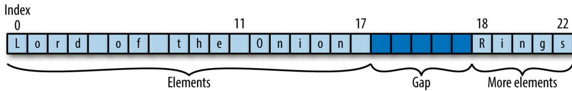
Figure 21-7. A gap buffer containing some more text
