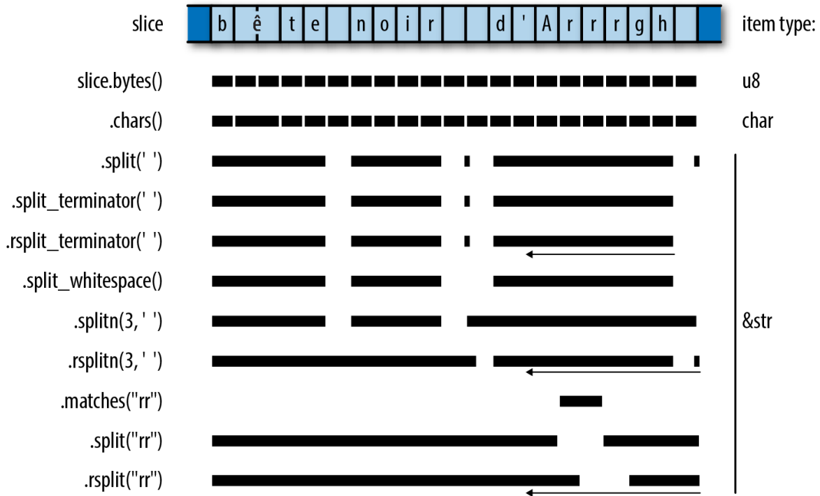
Figure 17-3. Some ways to iterate over a slice
