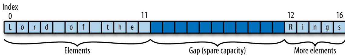
Figure 21-6. A gap buffer containing some text
