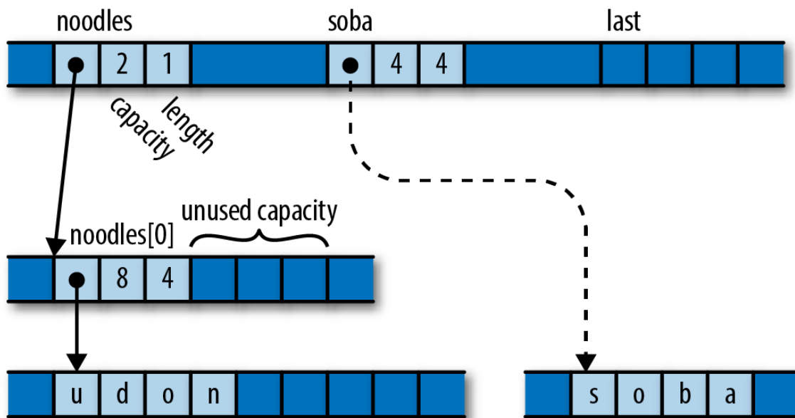
Figure 21-3. A vector with uninitialized, spare capacity
