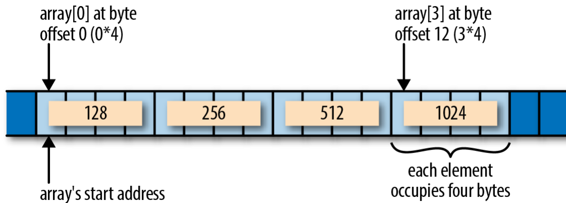
Figure 21-1. An array in memory
