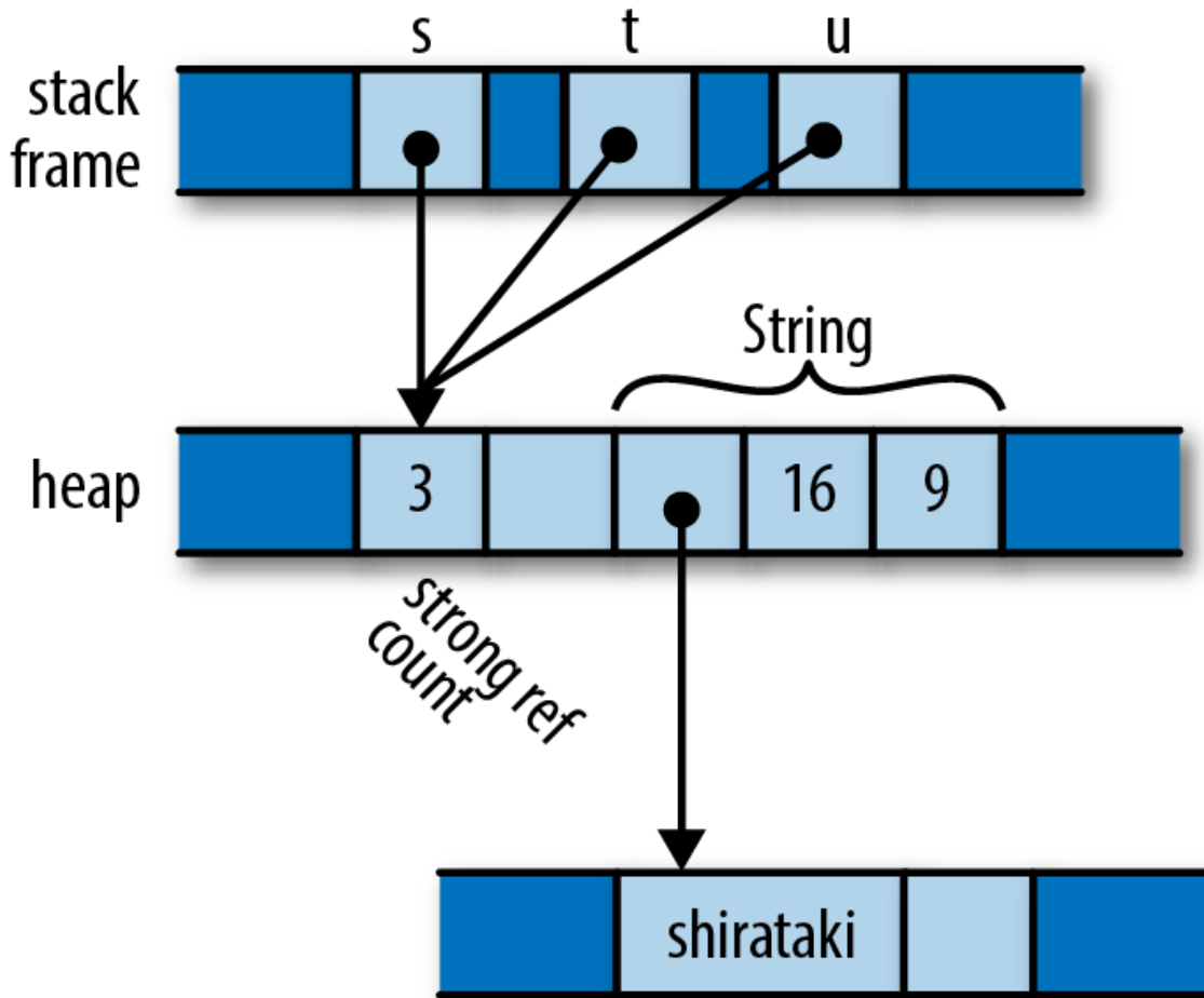
Figure 4-12. A reference-counted string, with three references
