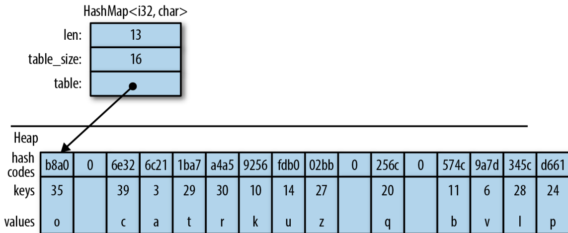
Figure 16-5. A HashMap in memory
