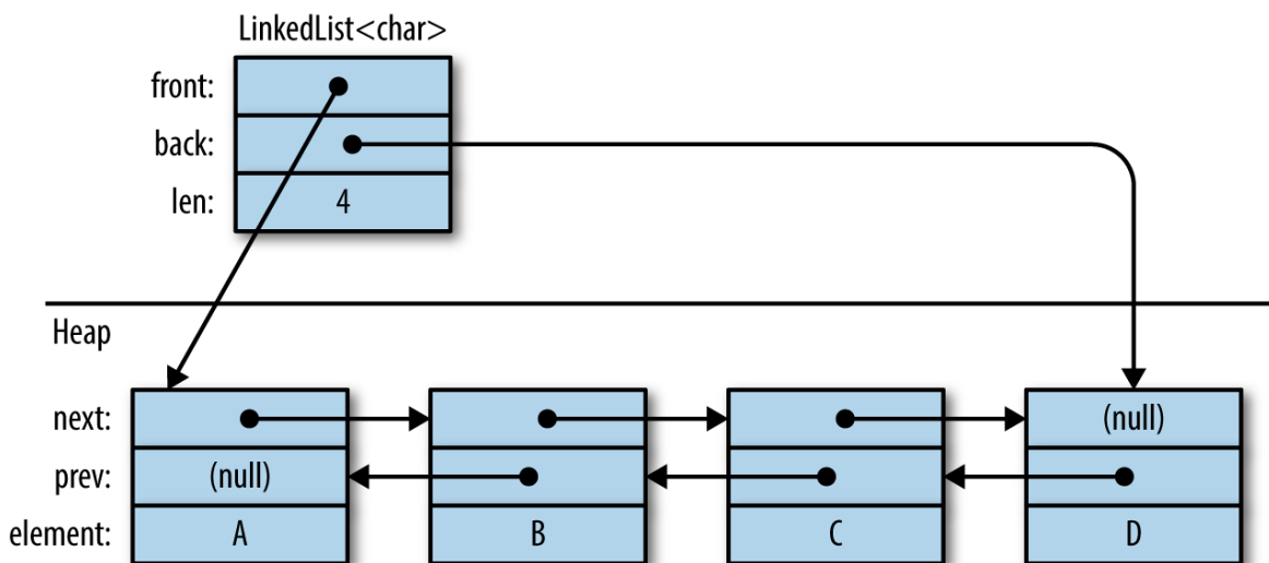
Figure 16-4. A LinkedList<char> in memory
