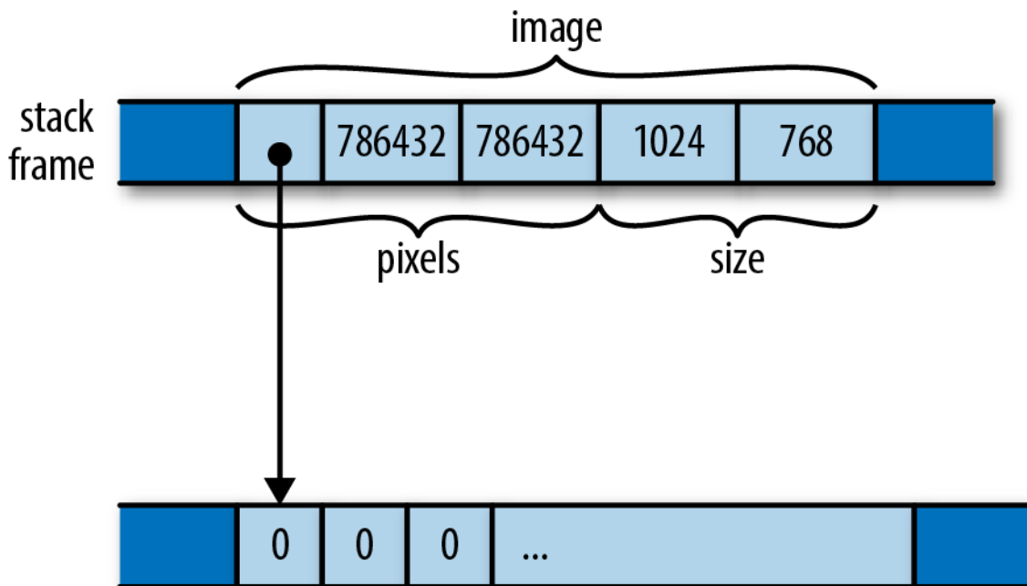
Figure 9-1. A GrayscaleMap structure in memory
