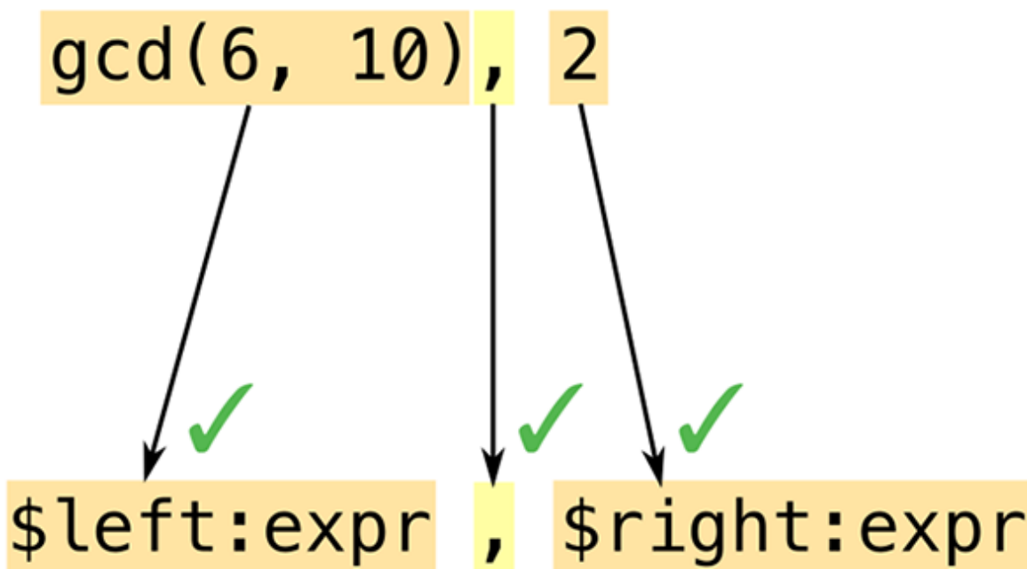
Figure 20-2. Expanding a macro, part 1: pattern matching on the arguments
