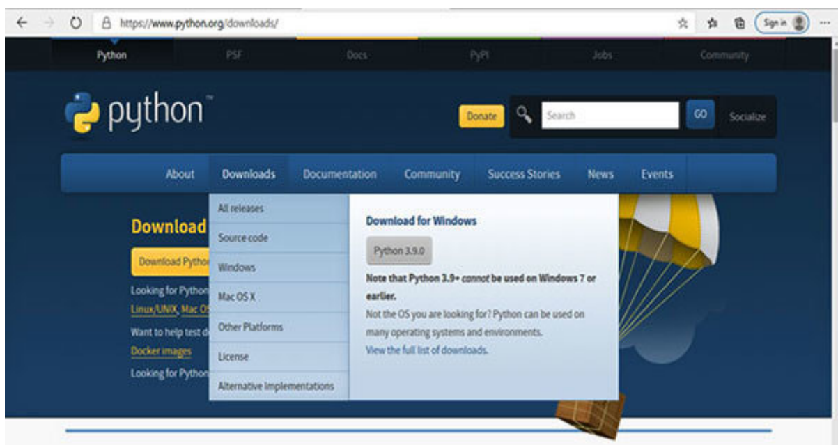
Figure 6.2: Downloading Python
