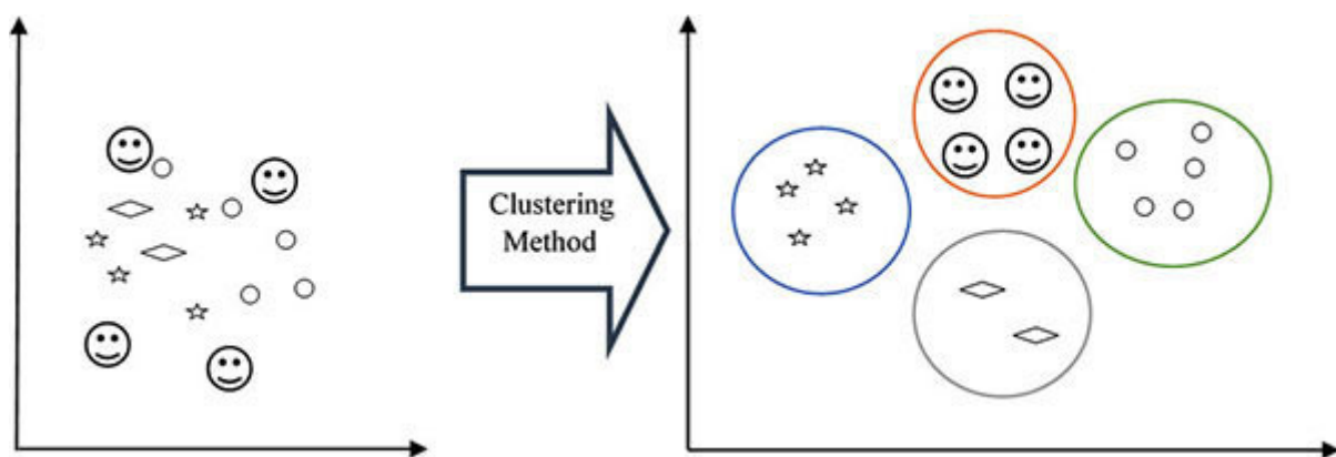
Figure 4.1: Clustering
