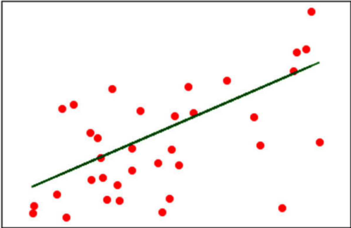
Figure 2.4: Simple Linear Regression for diabetes dataset
