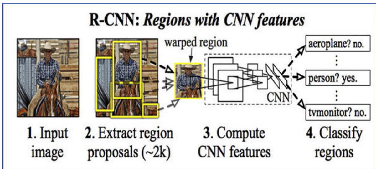
Figure 10.6: R-CNN model architecture
