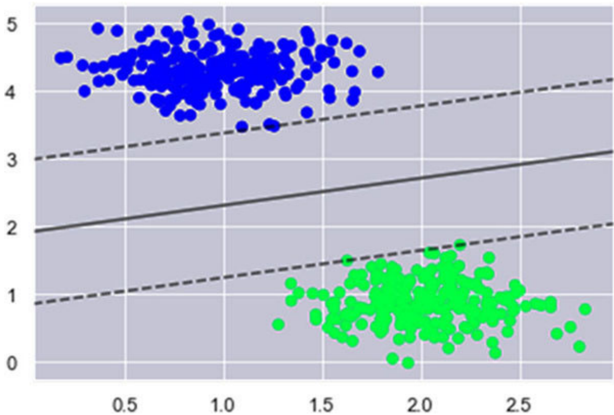
Figure 2.14: Decision function for 2-D SVC
