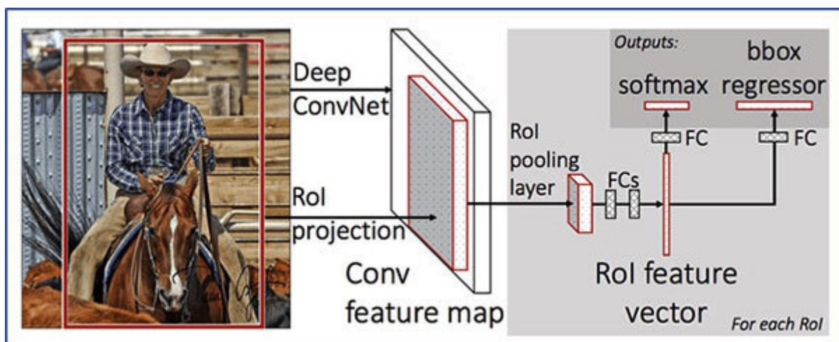
Figure 10.7: Fast R-CNN model architecture
