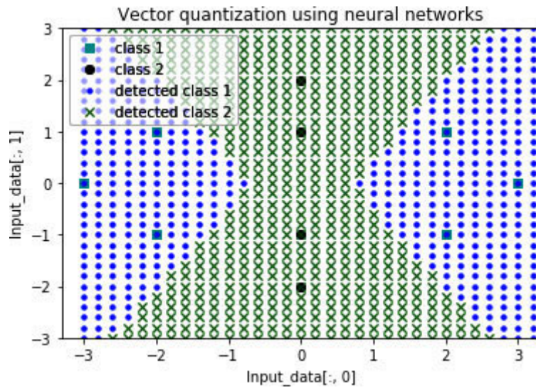
Figure 8.15: Vector quantization using neural networks
