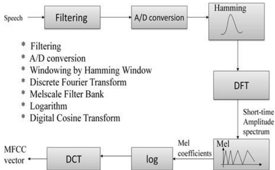
Figure 7.2: Block diagram of MFCC
