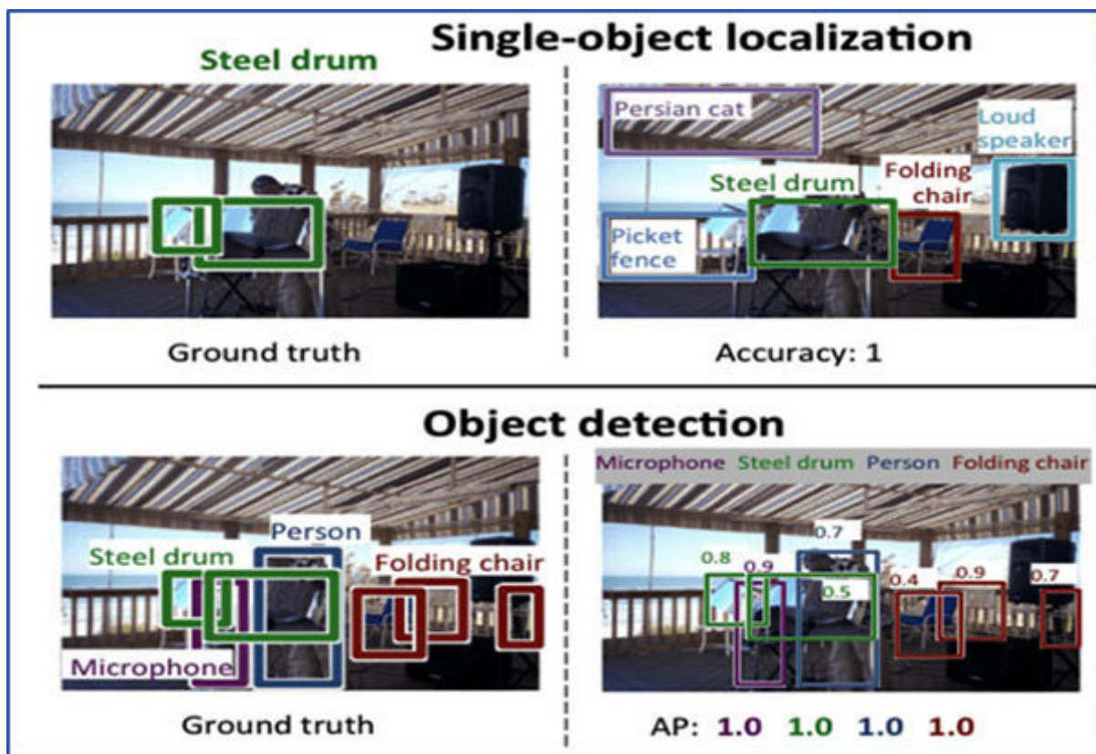
Figure 10.5: Comparison between single-object localization and object detection
