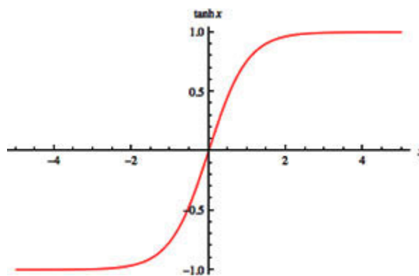
Figure 8.6: Tanh activation function
