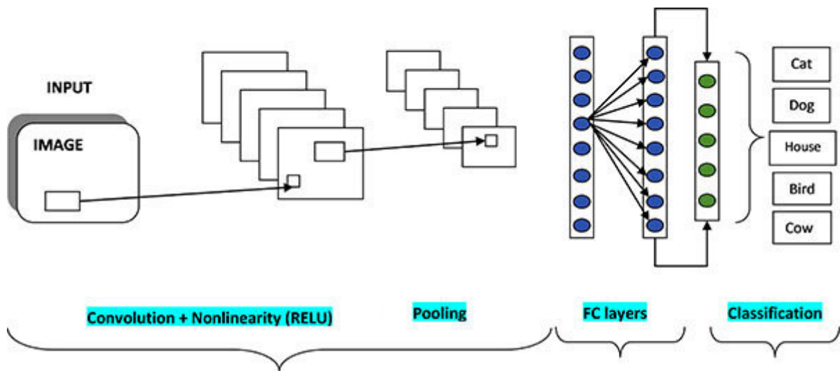
Figure 10.3: Architecture of CNN
