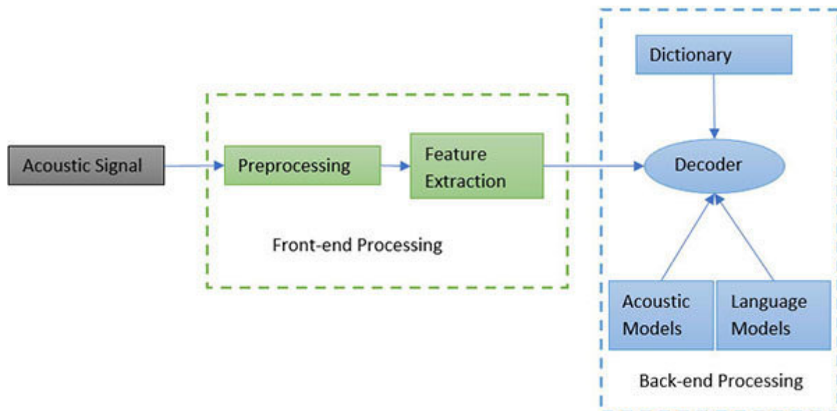
Figure 7.1: Structure of speech recognition system
