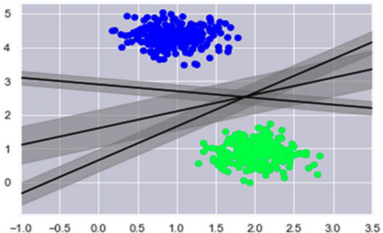
Figure 2.13: Discriminative Classification with margin of width
