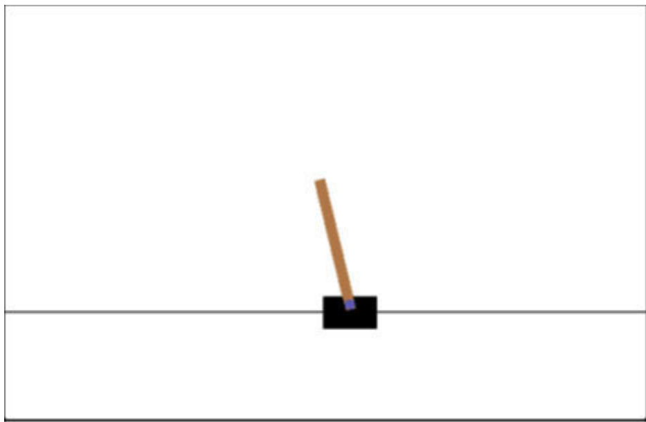
Figure 9.5: CartPole environment-screenshot1
