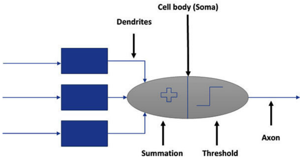
Figure 8.2: Model of a biological neuron
