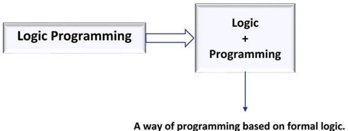
Figure 5.1: Logic Programming
