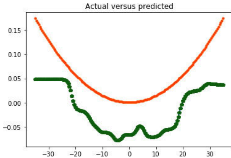
Figure 8.14: Actual versus predicted output (multi-layer neural network)
