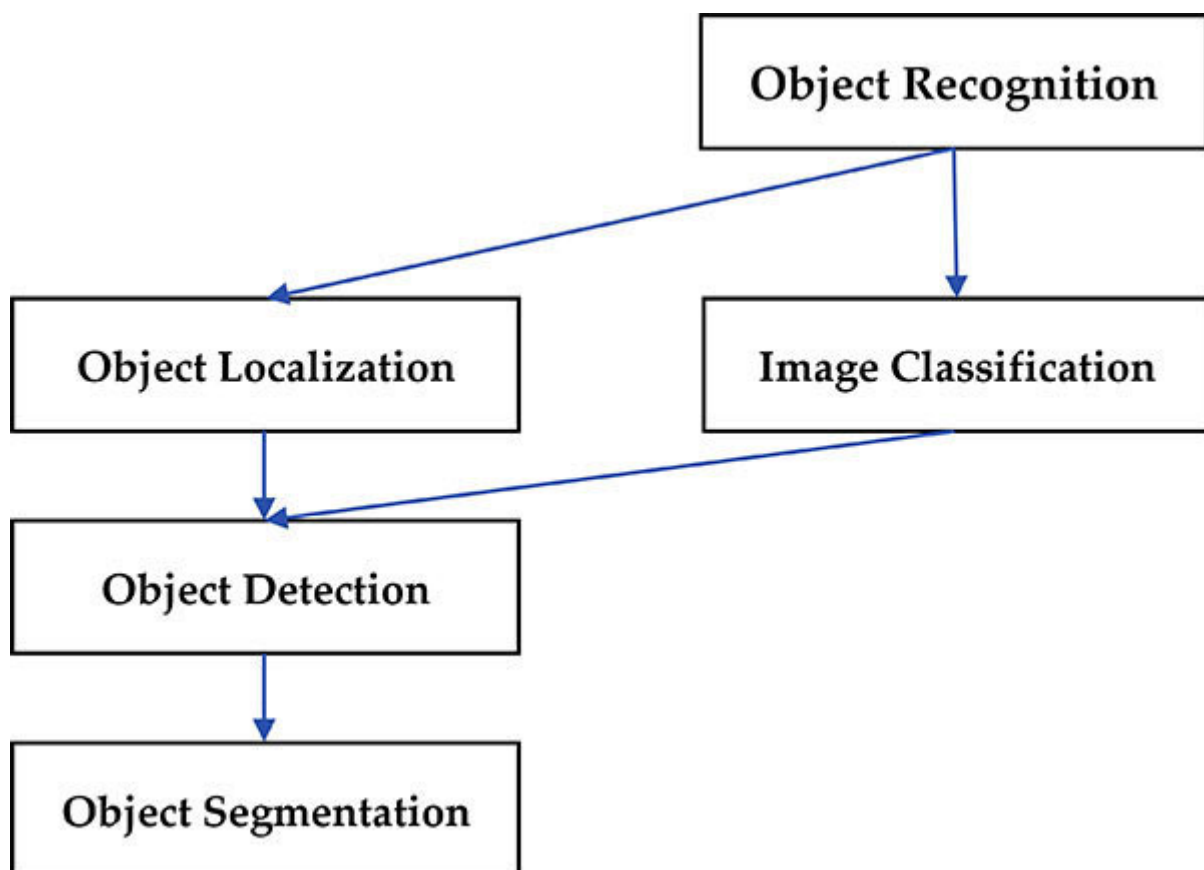
Figure 10.4: Object recognition computer vision tasks
