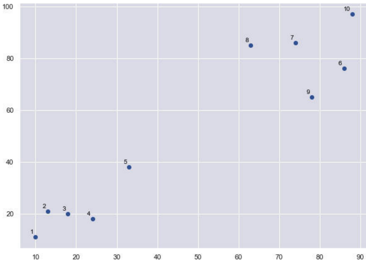
Figure 4.10: Data points
