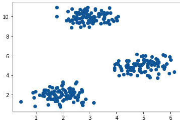
Figure 4.8: Sample dataset
