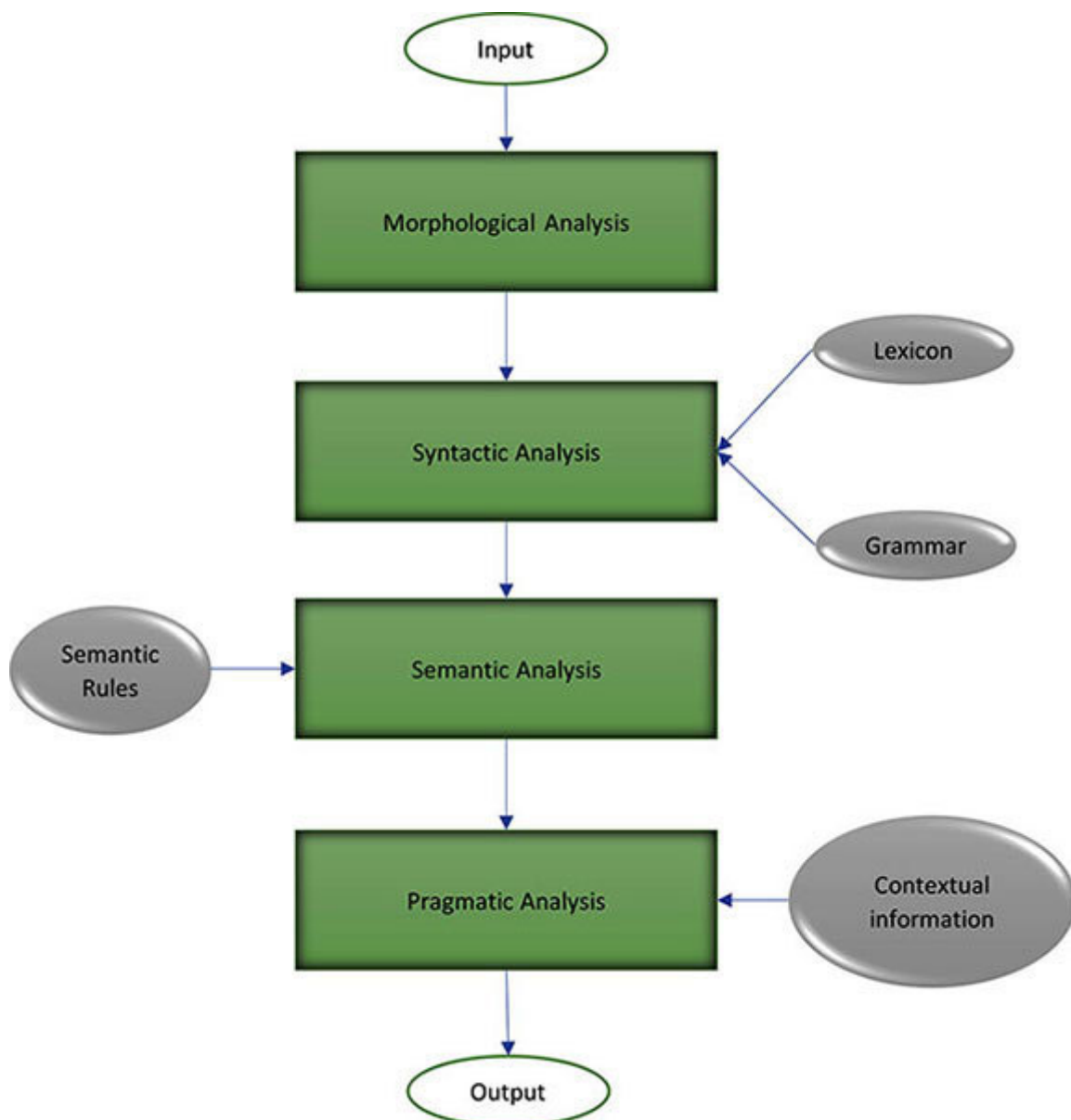
Figure 6.1: NLP phases
