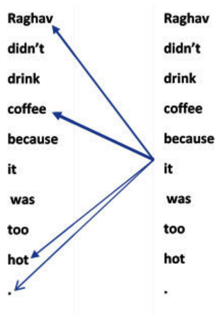
Figure 6.9: Understanding self-attention
