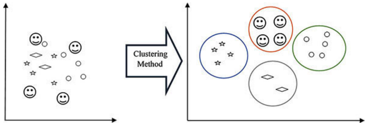
Figure 2.2: Clustering Method
