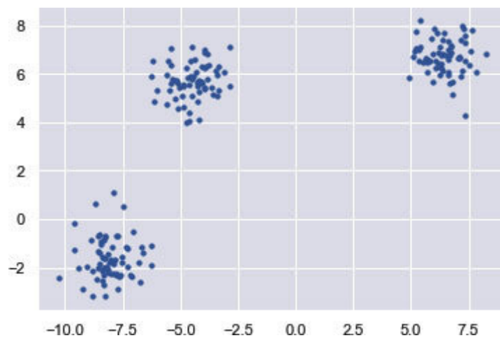
Figure 4.5: Data having 3-blobs
