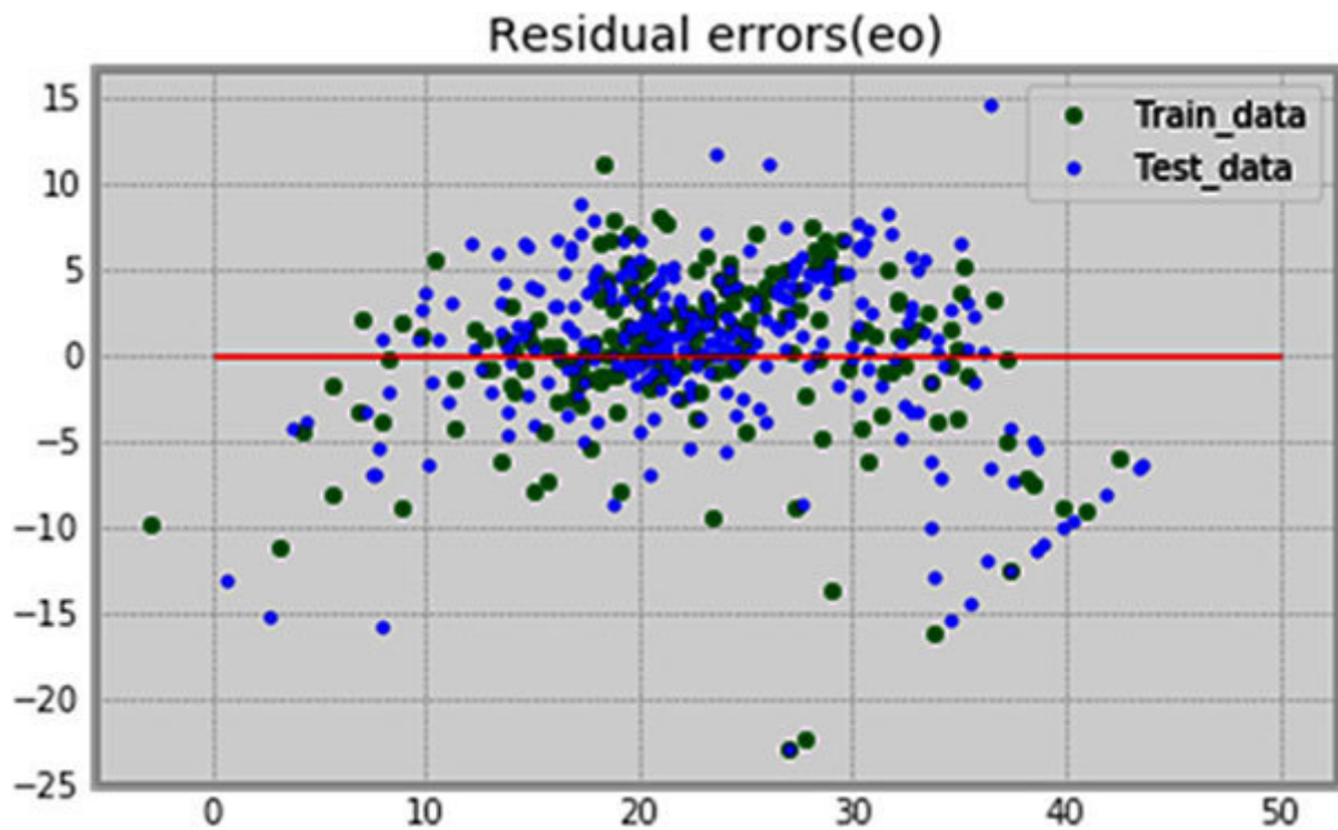
Figure 2.5: Multiple Linear Regression
