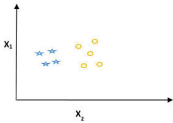
Binary Classification
