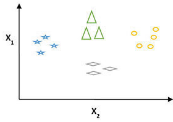
Multi-class Classification
