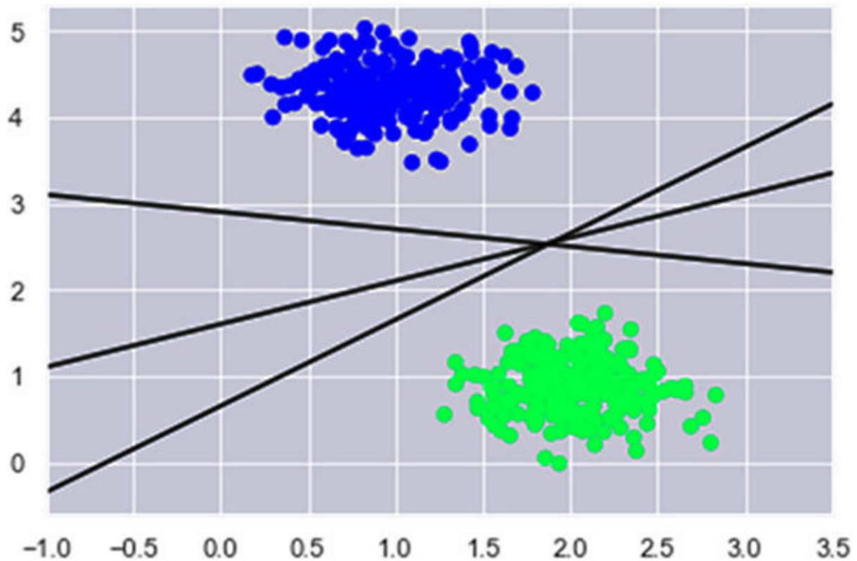
Figure 2.12: Discriminative Classification
