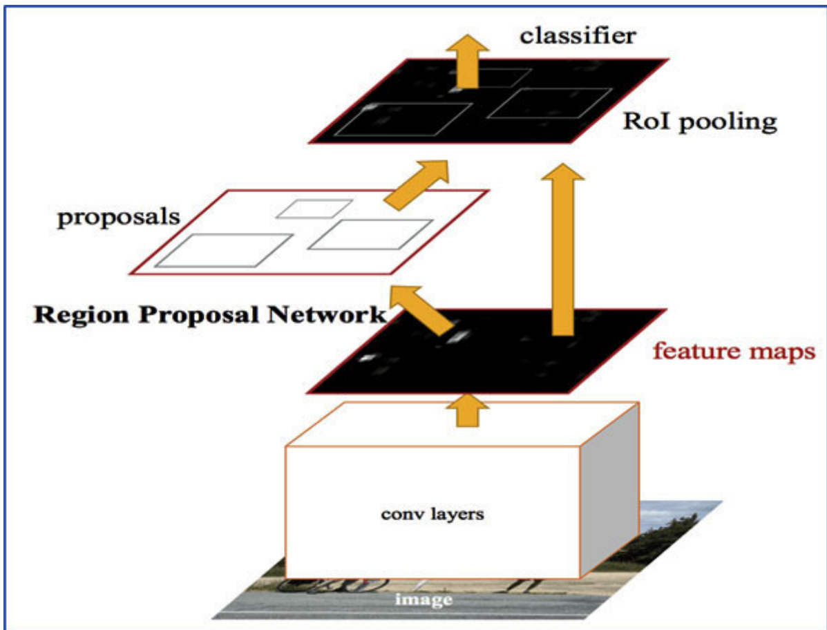
Figure 10.8: Faster R-CNN model architecture
