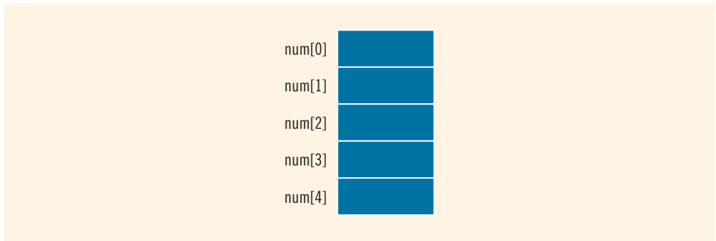
FIGURE 8-1 Array num
