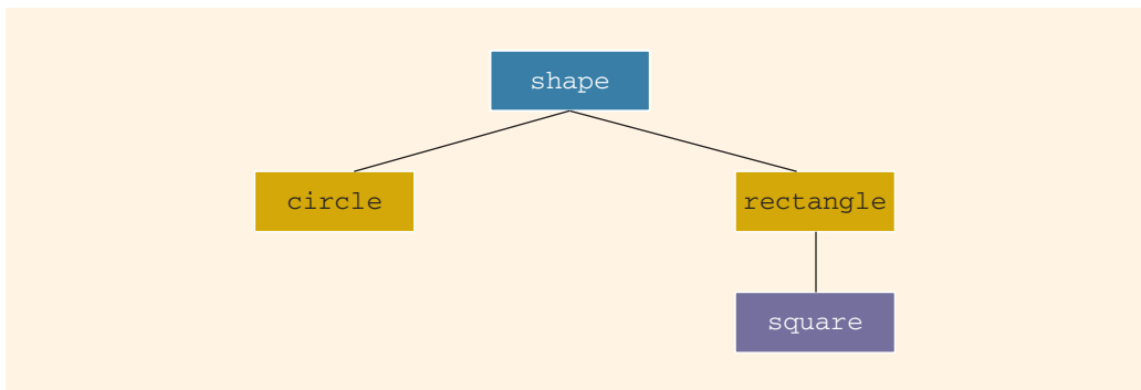
FIGURE 11-1 Inheritance hierarchy
