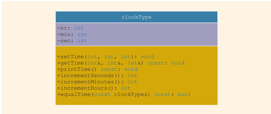
FIGURE 10-1 UML class diagram of the class clockType
