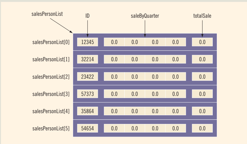
FIGURE 9-10 Array salesPersonList after initialization
