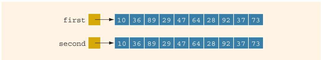
FIGURE 12-12 first and second both pointing to their own data
