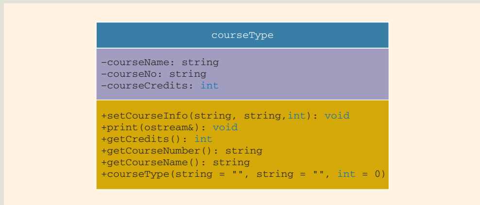
FIGURE 11-9 UML class diagram of the class courseType
