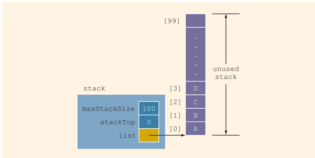
FIGURE 18-7 Empty stack
