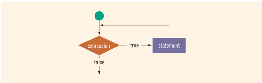
FIGURE 5-1 while loop
