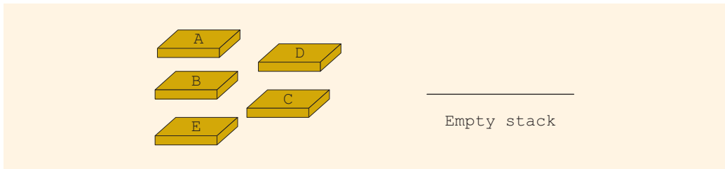
FIGURE 18-2 Empty stack
