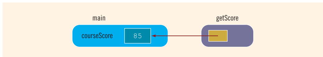
FIGURE 6-6 Variable courseScore and the parameter score after the statement in Line 5 executes
