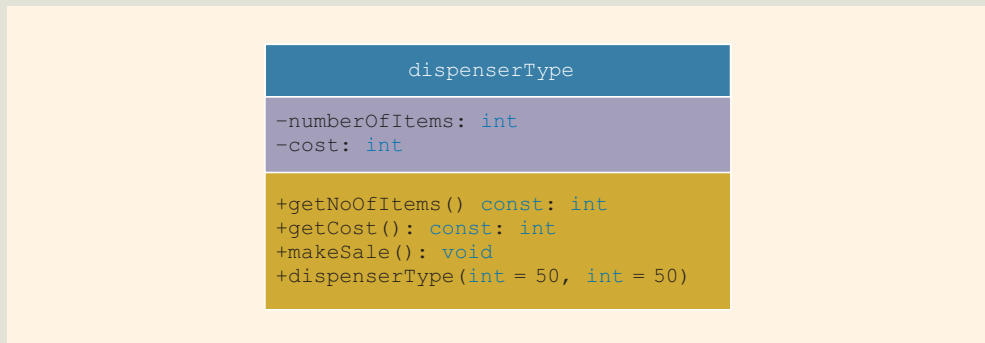
FIGURE 10-16 UML class diagram of the class dispenserType
