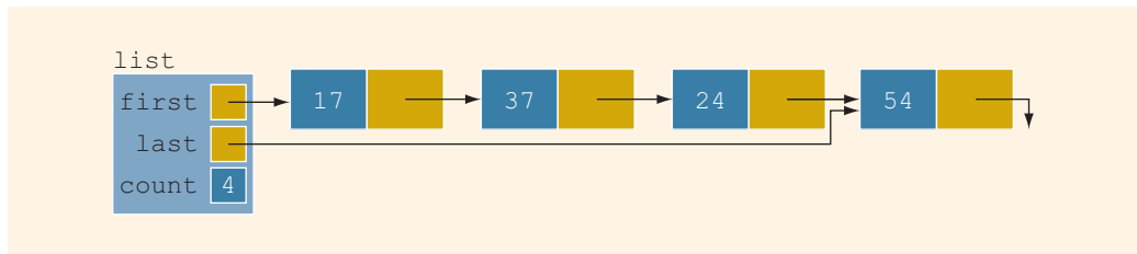
FIGURE 17-24 list after deleting node with info 28
