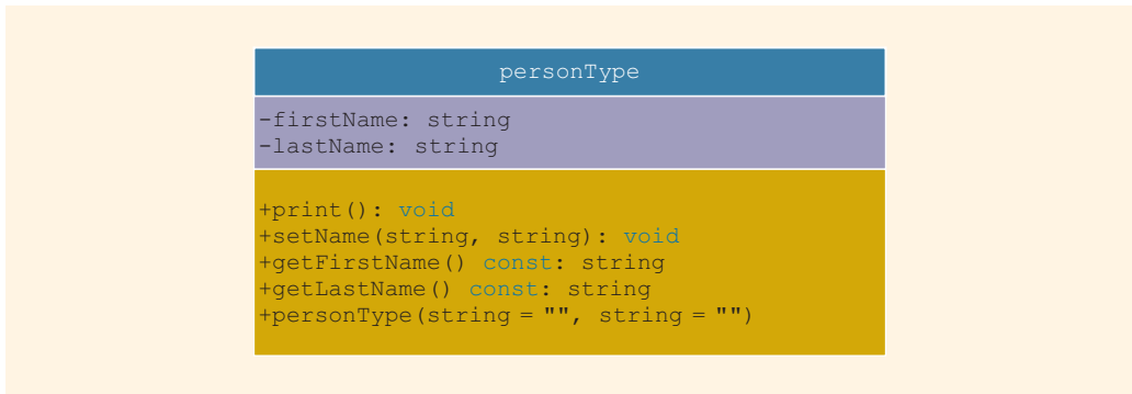
FIGURE 10-11 UML class diagram of the class personType
