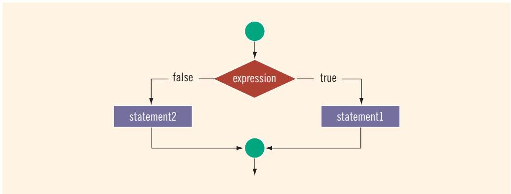
FIGURE 4-3 Two-way selection
