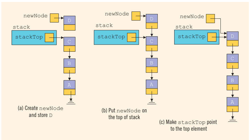
FIGURE 18-14 Push operation
