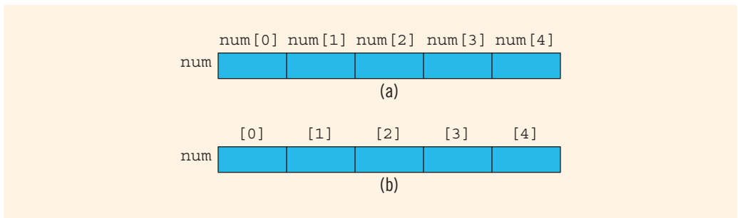
FIGURE 8-2 Array num
