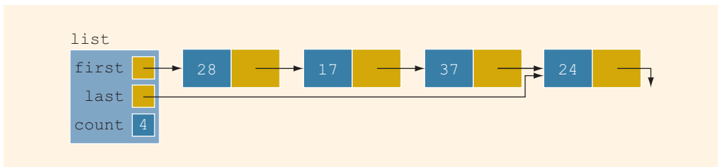
FIGURE 17-28 list after deleting 54
