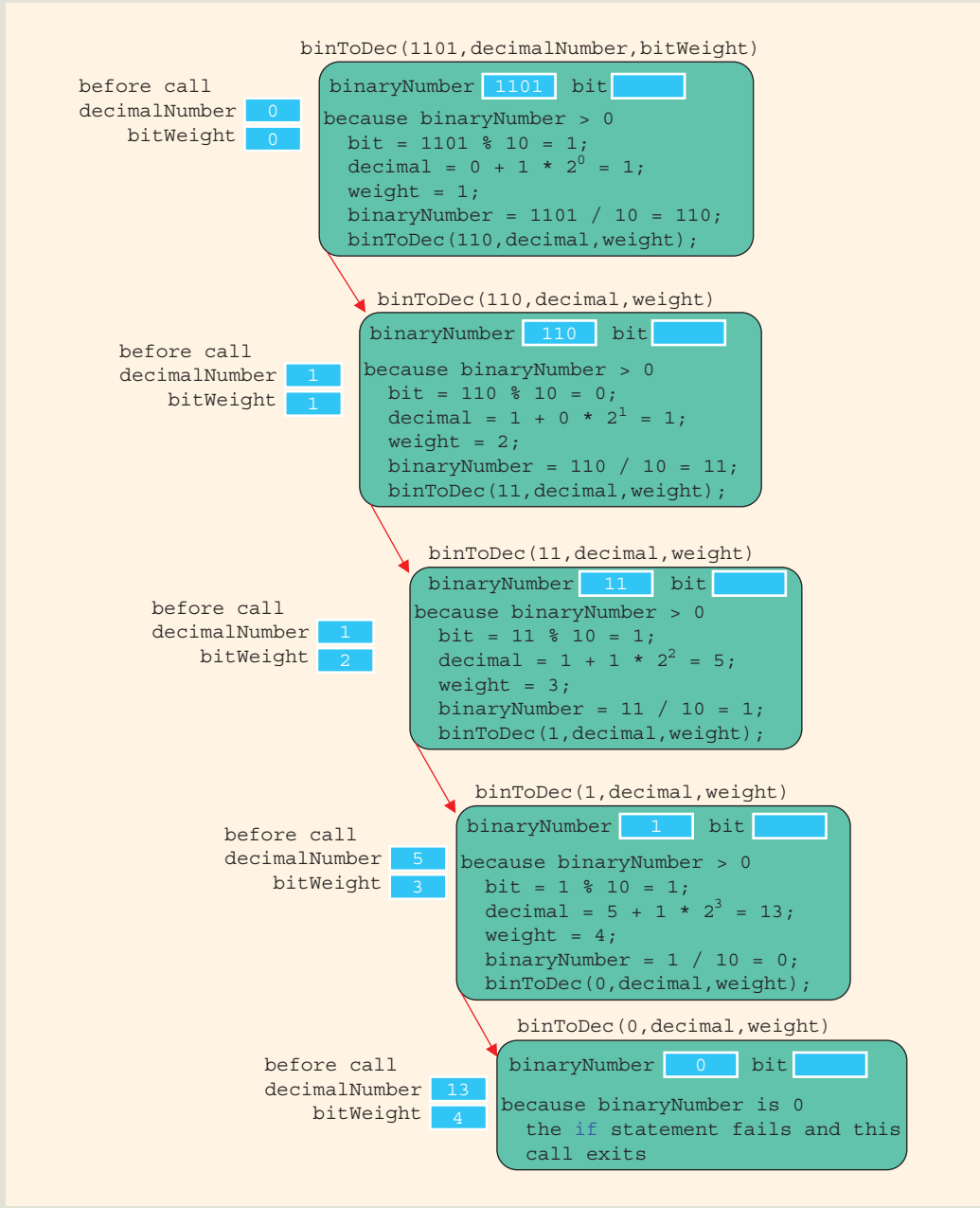
FIGURE 15-8 Execution of binToDec(1101, decimalNumber, bitWeight);
