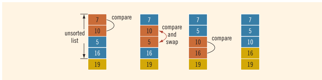
FIGURE 16-3 Elements of list during the second iteration
