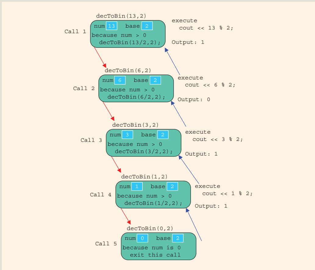
FIGURE 15-9 Execution of decToBin(13, 2)
