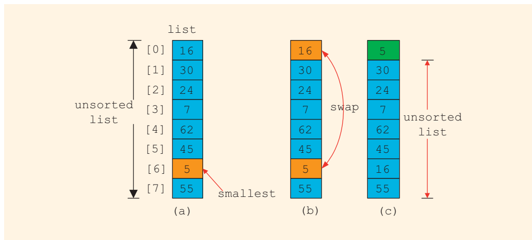
FIGURE 8-10 Elements of list during the first iteration
