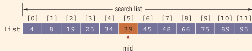
FIGURE 16-14 Search list, list[0]...list[11]
