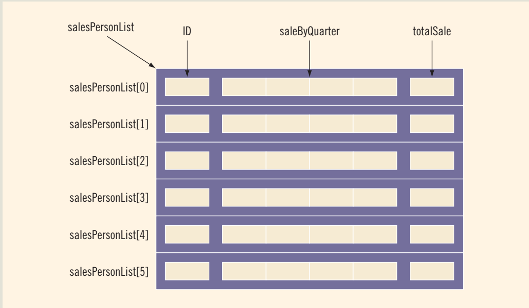
FIGURE 9-9 Array salesPersonList
