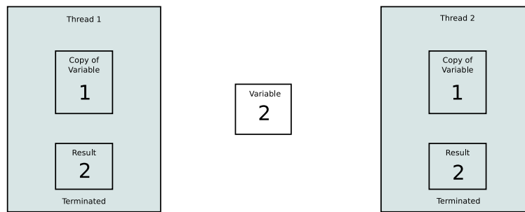
Figure 63: Both Threads Terminated
