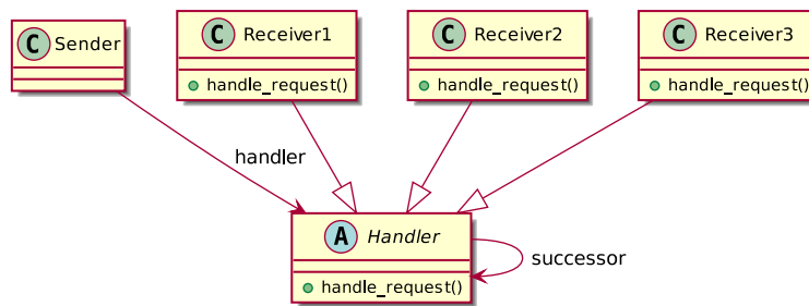
Figure 124: UML Diagram of the Chain of Responsibility Pattern
