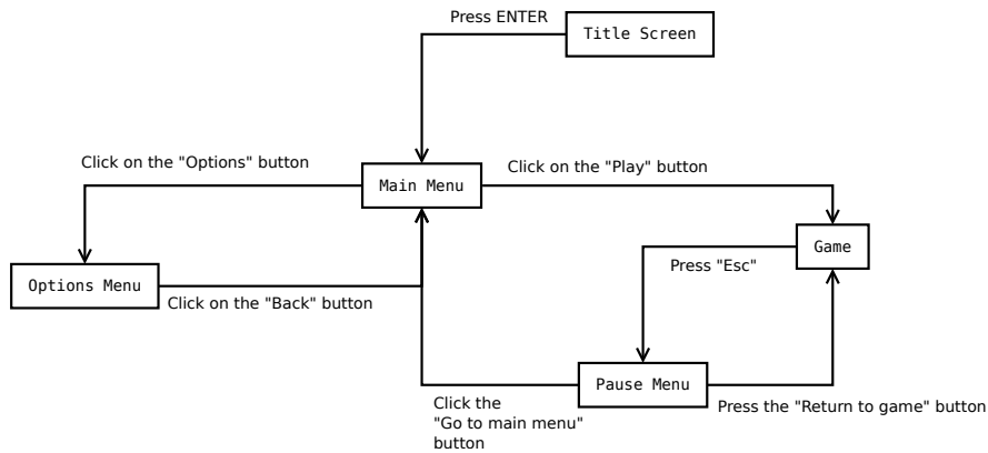
Figure 127: Diagram of a menu system's state machine
