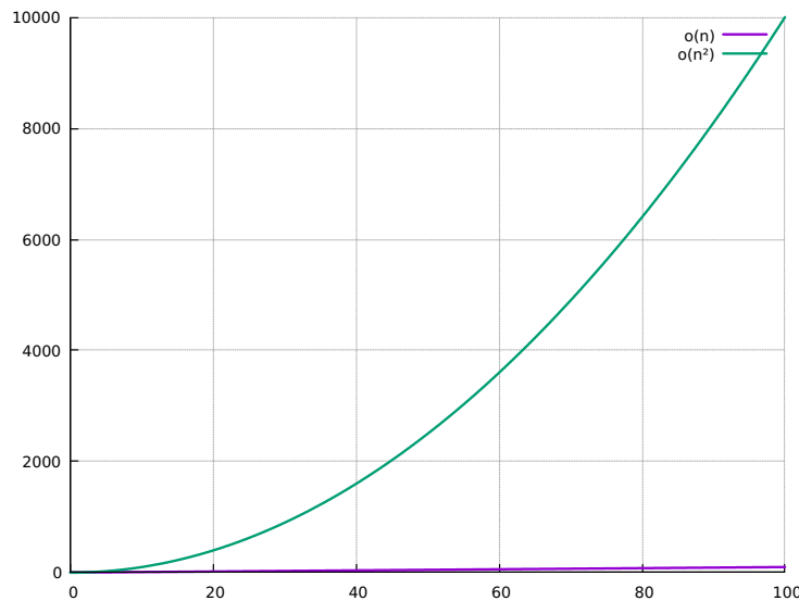
Figure 10: O(n) growth rate, compared to O(n^2)
