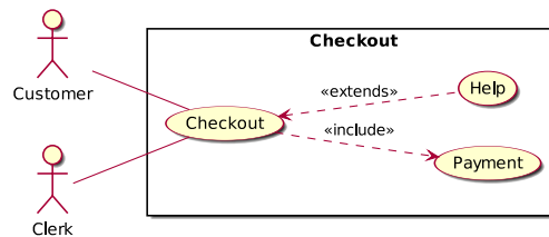
Figure 20: Example of a sub-use case
