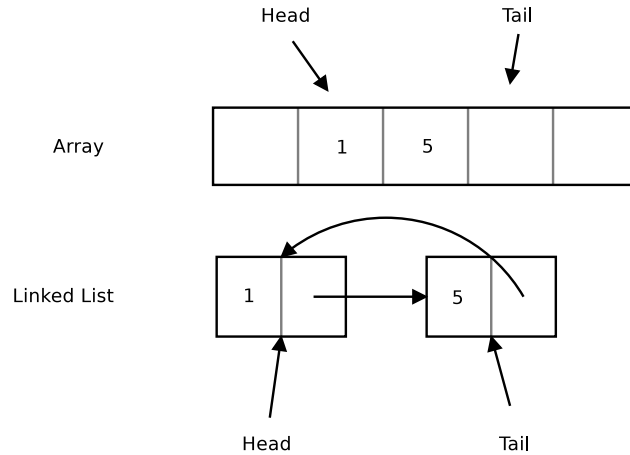
Figure 57: Array and linked list implementation of a circular queue
