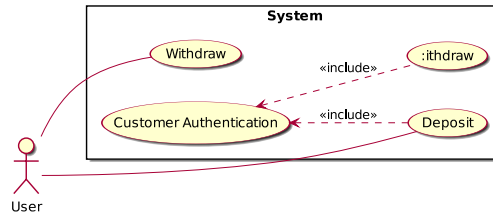
Figure 19: Example of a use case inclusion
