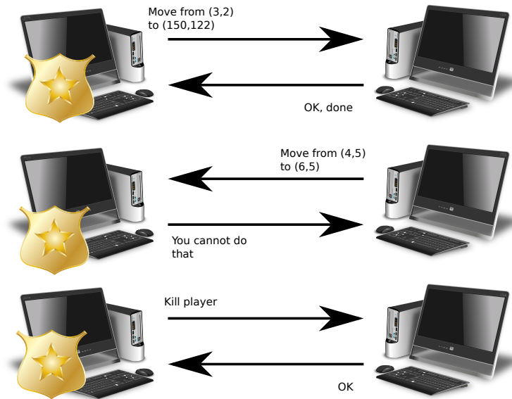
Figure 176: What would happen if one of the Peers had the authoritative game state
