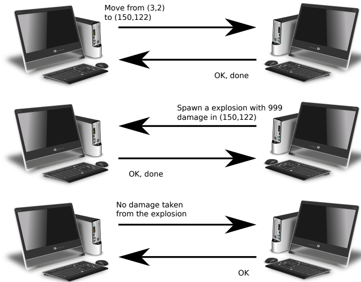
Figure 175: Two cheaters meet in P2P
